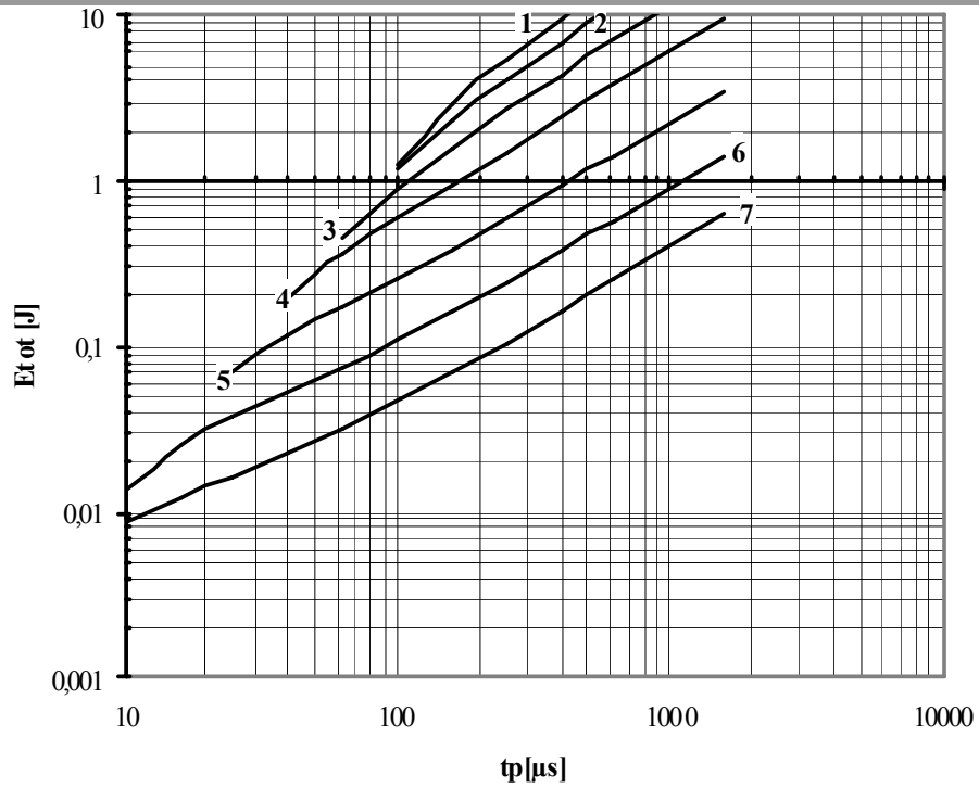
Fig. 24 Square wave loss energy per pulse
