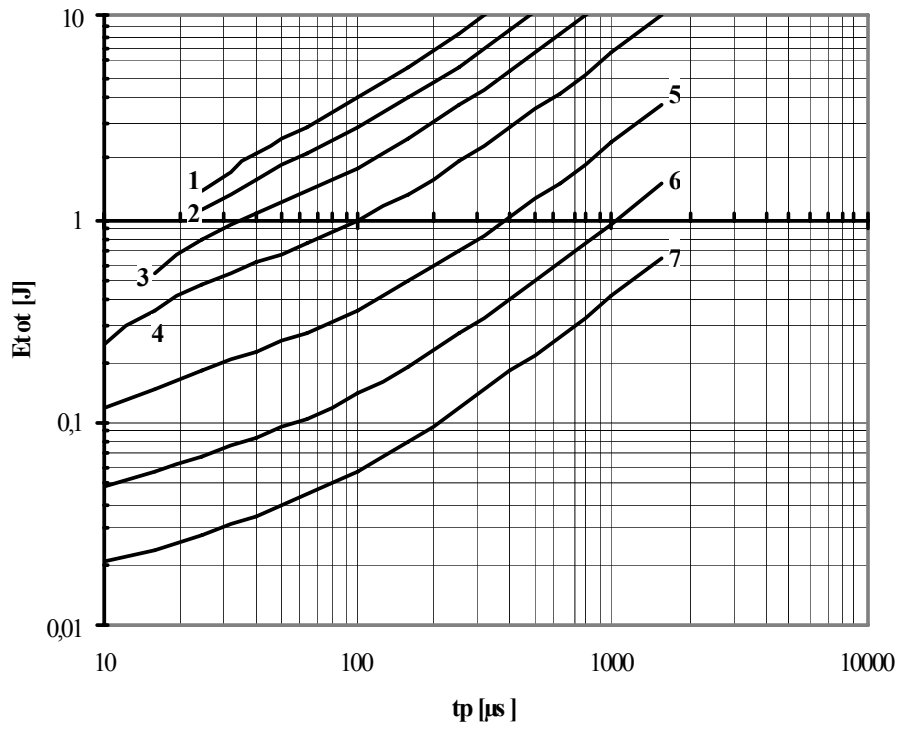
Fig. 25 Square wave loss energy per pulse
