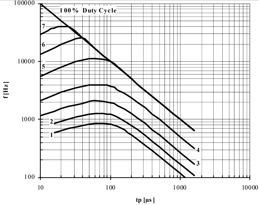
Fig. 12 Sine wave frequency ratings
